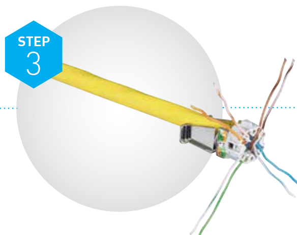
Separate and insert the pairs
