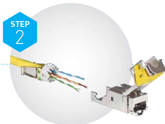
Pass the cable through the back of the wire housing
